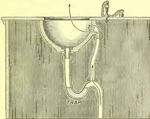
FIG. 26.—A typical basin. ("Sanitary Engineer.")
